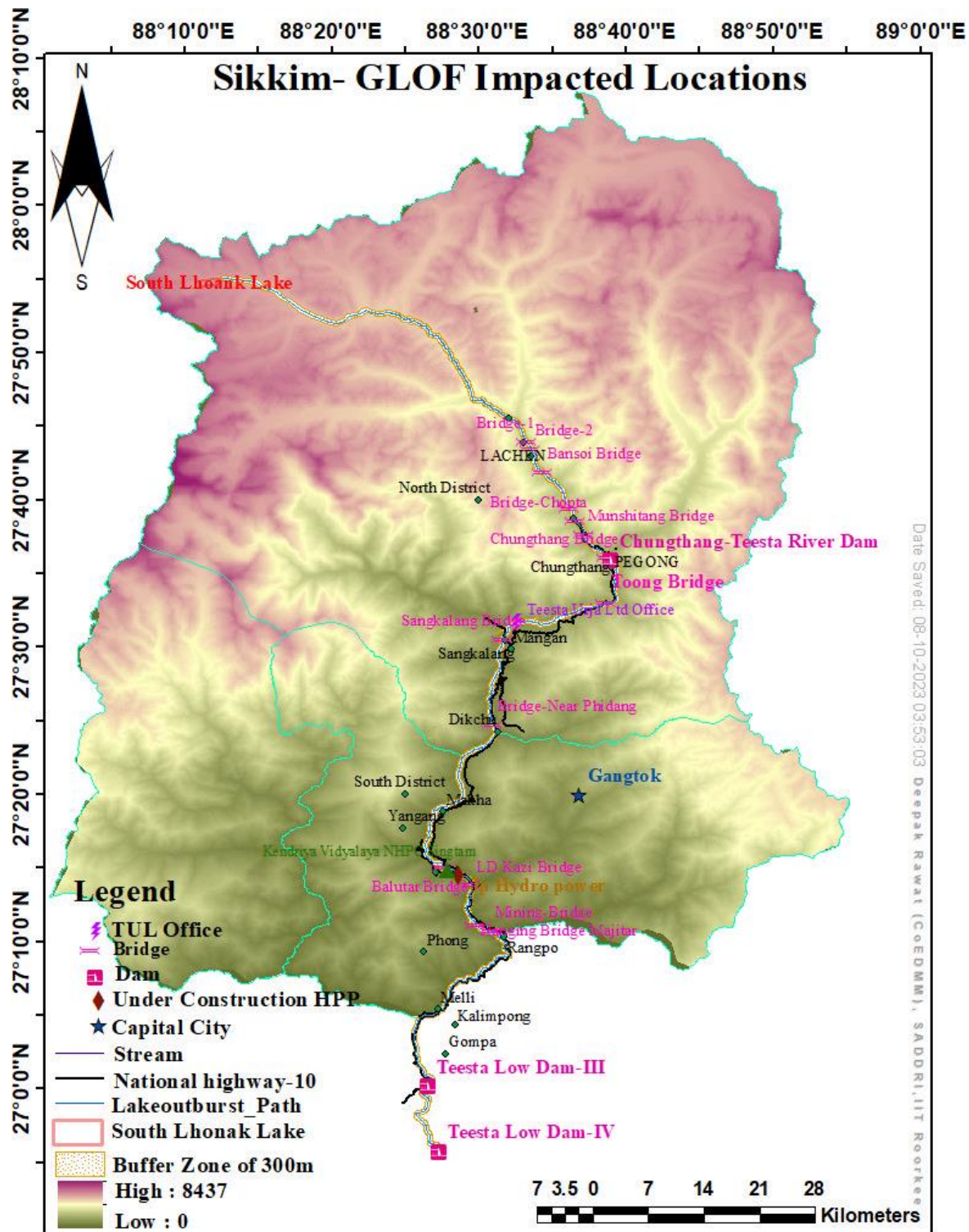
Figure.1 South Lhonak Lake serves as the point of origin for the catastrophic flood event, and the subsequent course of the flood extends along the Teesta River and National Highway 10. This trajectory reveals the specific areas heavily impacted by the flash flood, resulting in property damage and significant consequences. The figure provides a clear depiction of the vulnerability of this valley, highlighting the presence of critical infrastructure, including schools, in the affected region.
