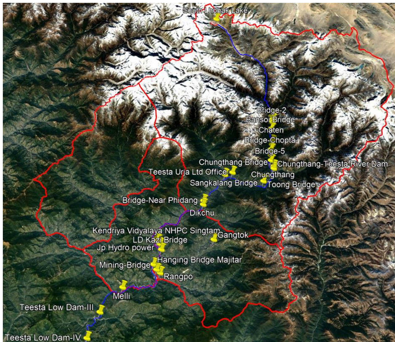
Figure. 2. Red border showing the Sikkim state and district boundaries. Blue line showing the path followed by the GLOF and along this path devastation have seen by flash flood and major critical place have been marked.
